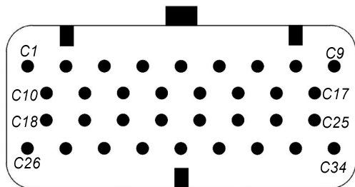
CONNECTOR C
