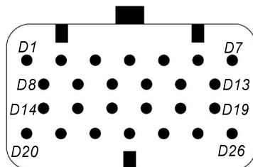
CONNECTOR D
