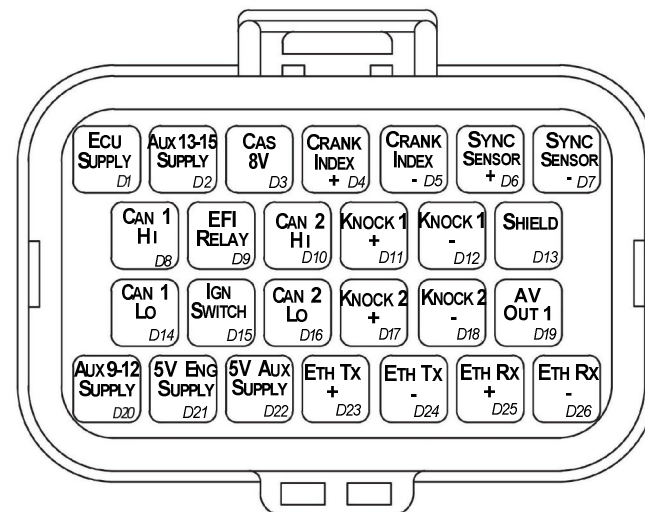
CONNECTOR D
