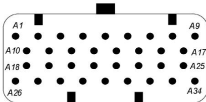
CONNECTOR A
