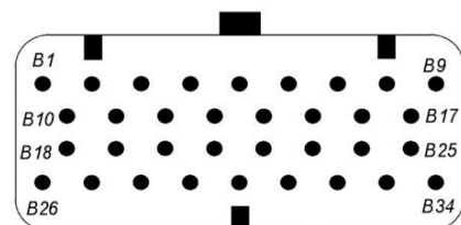
CONNECTOR B
